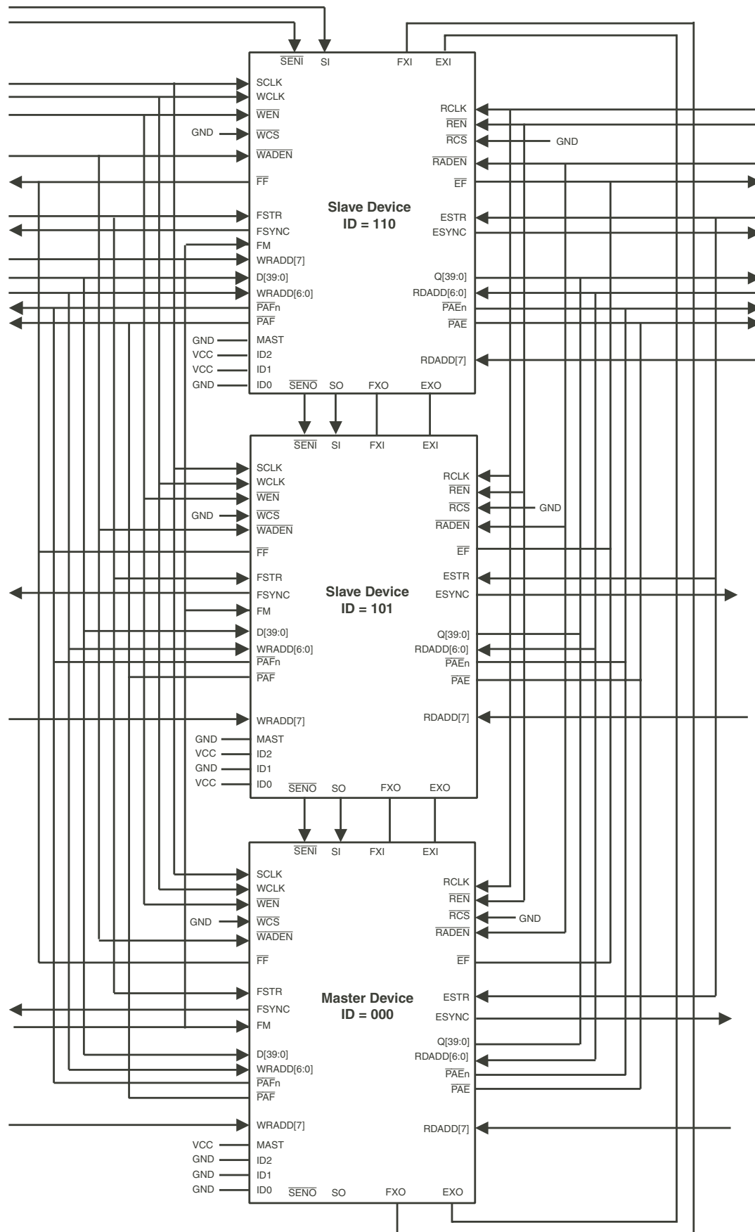
Figure 62. Connecting THREE or more 10G MQ 128Q in Expansion Mode Using WADDR bit 7/RDADDR bit 7
