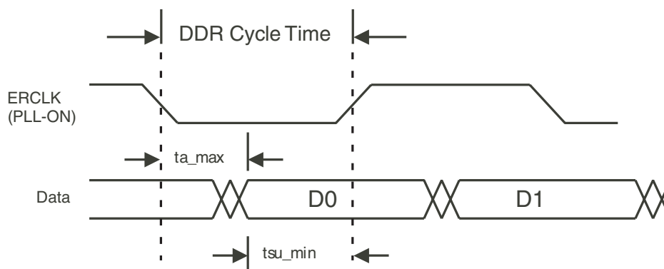
Figure 34. DDR Source Synchronous Center Aligned Clocking
