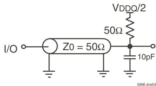
Figure 2a. AC Test Load
