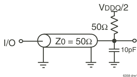
Figure 5a. AC Test Load
