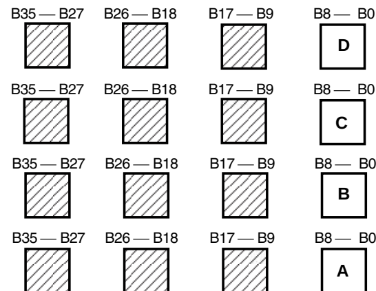
Figure 2. Bus sizing
