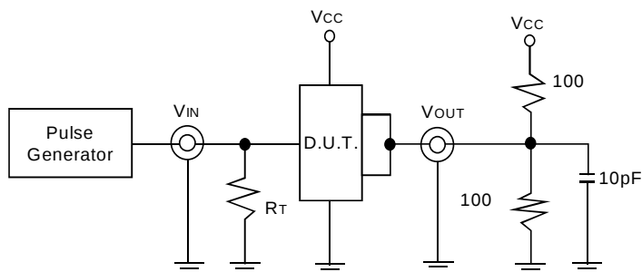
Figure 1. Z_o = 50\Omega to V_{cc}/2 , C_L = 10\text{pF}
