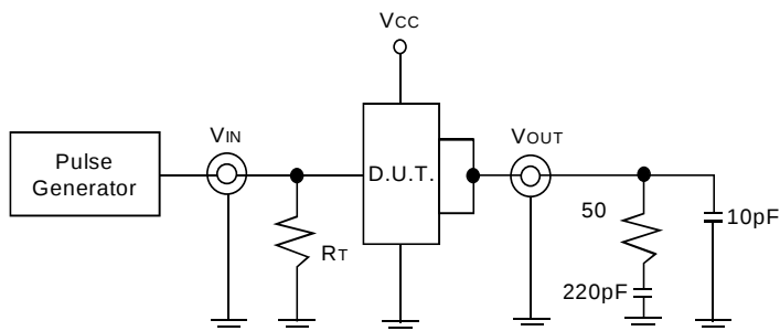
Figure 2. Z_o = 50\Omega AC Termination, C_L = 10\text{pF}
