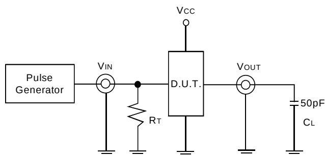
Figure 3. C_L = 50\text{pF} Circuit
