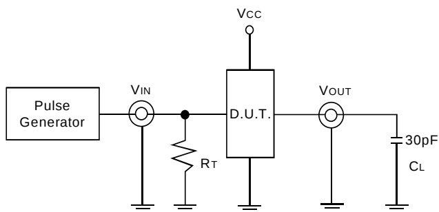
Figure 3. C_L = 30\text{pF} Circuit
