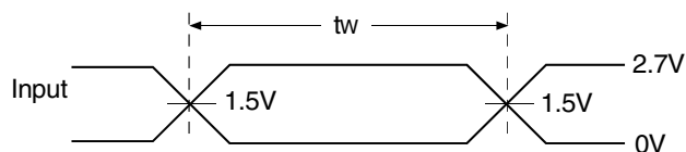
Voltage Waveforms Pulse Duration
