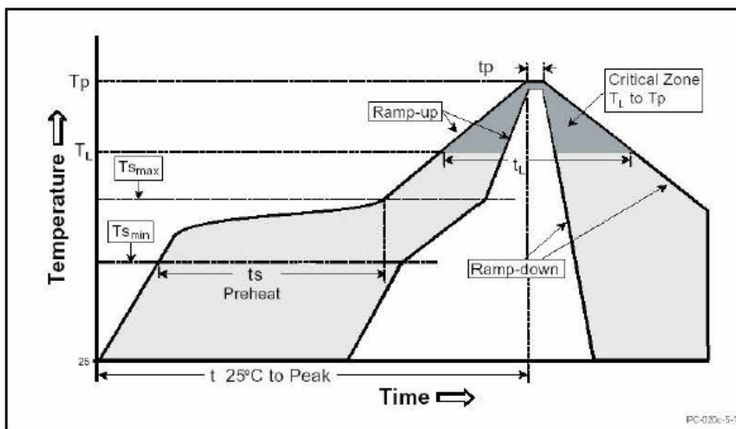
Figure 15. Solder Reflow Profile
