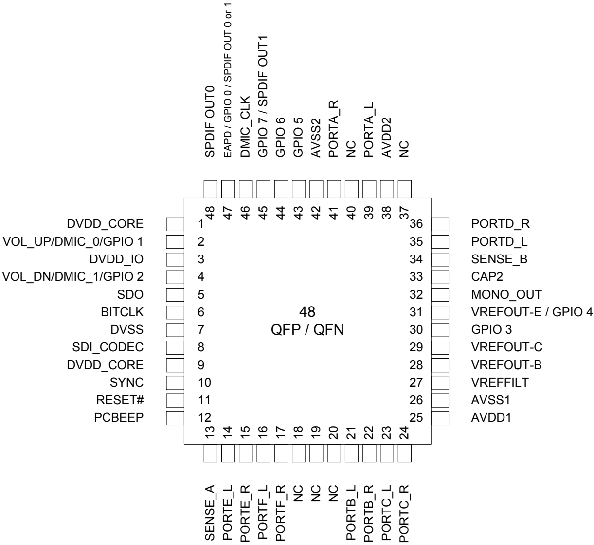
Figure 12. Pin Assignment
