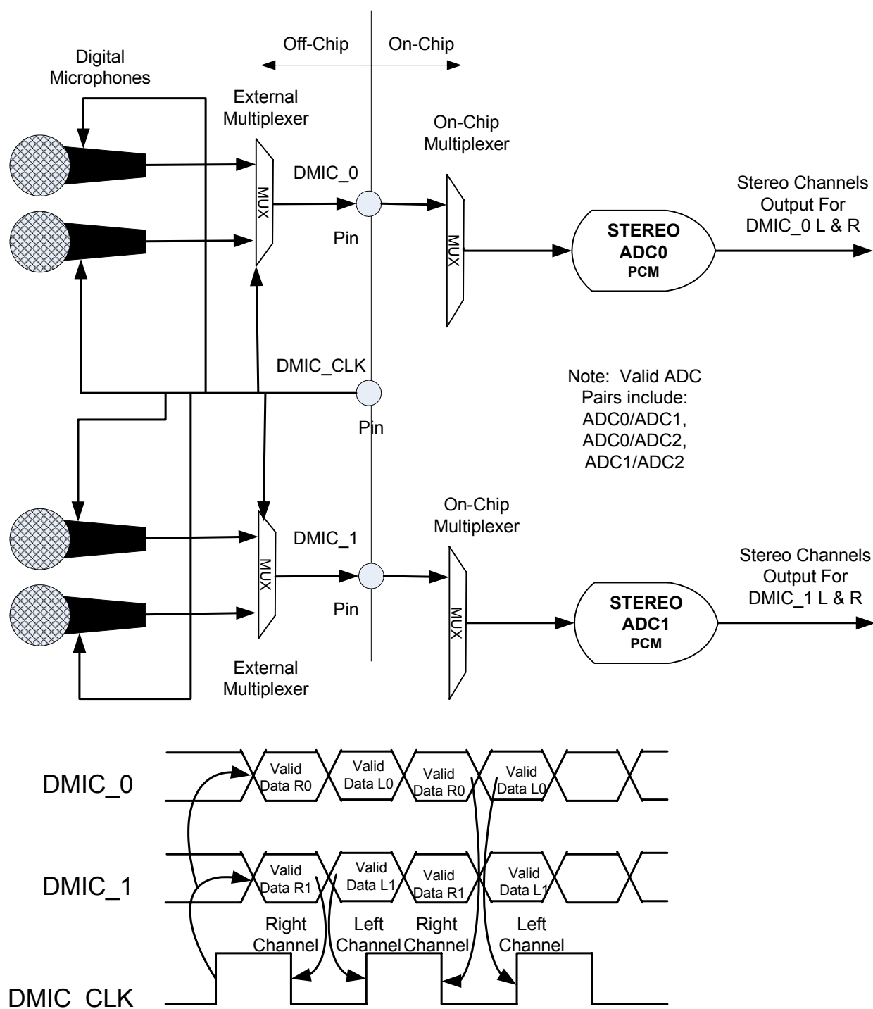
Figure 3. Quad Digital Microphone Configuration
