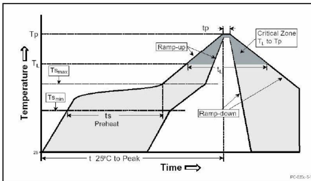
Figure 6. Reflow Profile
