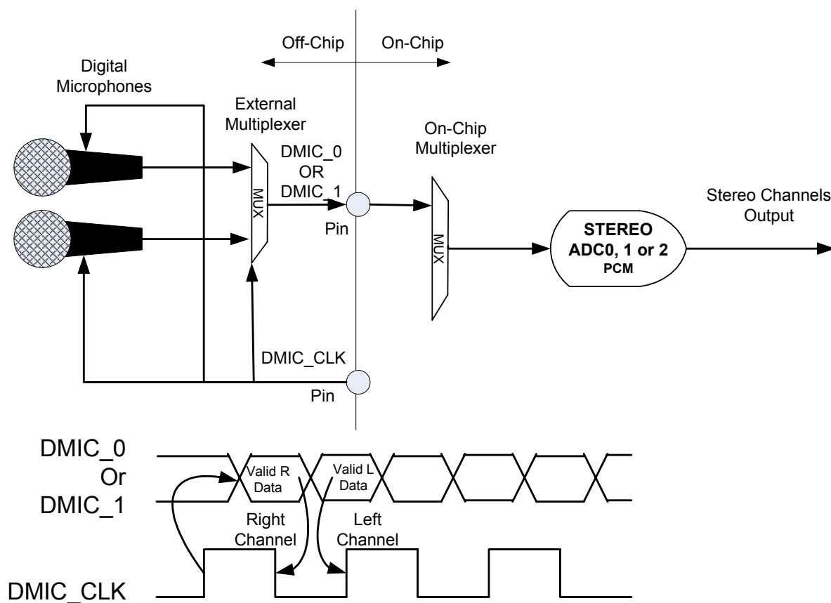
Figure 2. Stereo Digital Microphone Configuration
