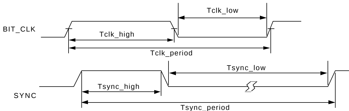
Figure 4. Clocks Timing
