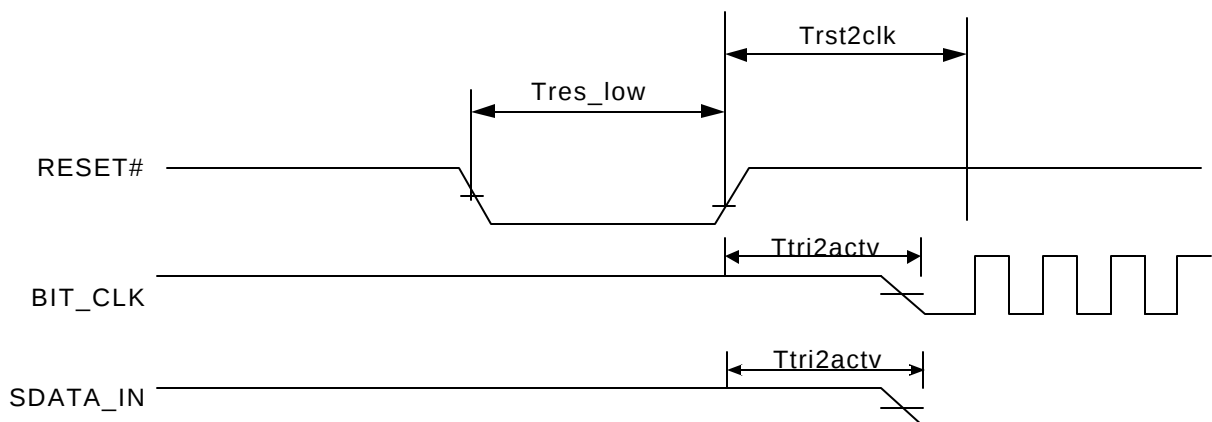
Figure 2. Cold Reset Timing
