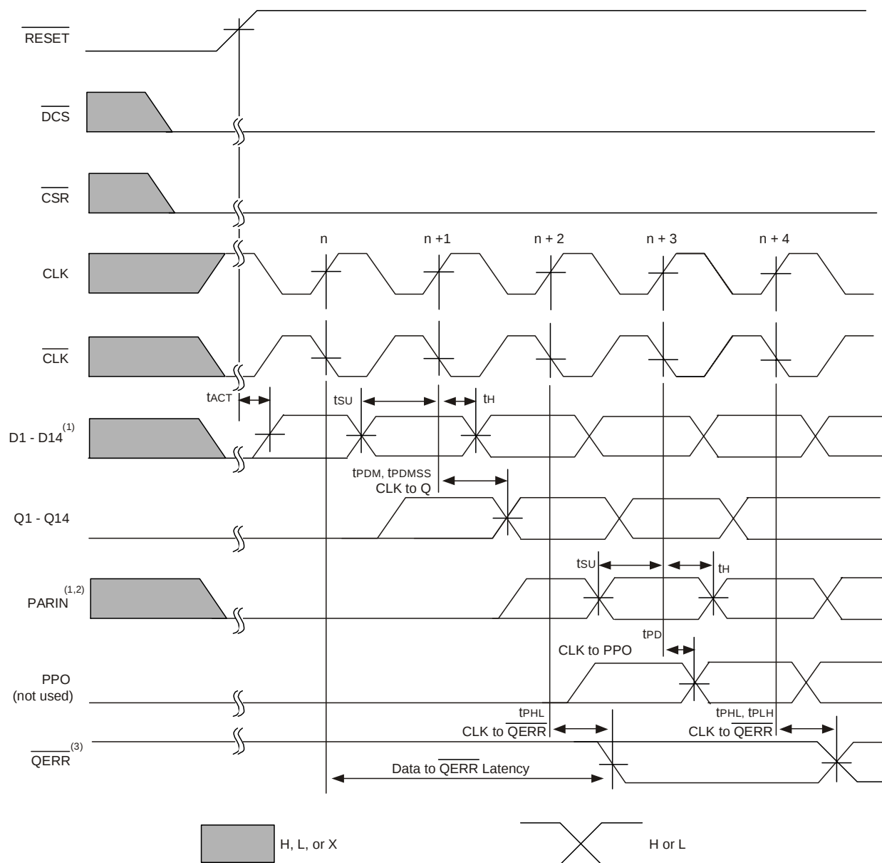
Timing Diagram for the Second SSTUAF32866B (1:2 Register-B Configuration) Device Used in a Pair; C0 = 1, C1 = 1, \overline{RESET} Switches from L to H
