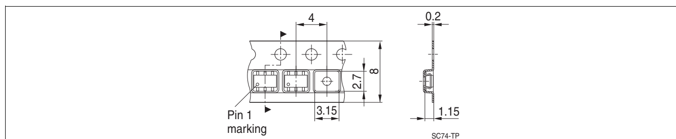
Figure 16 PG-SC74: Packing
