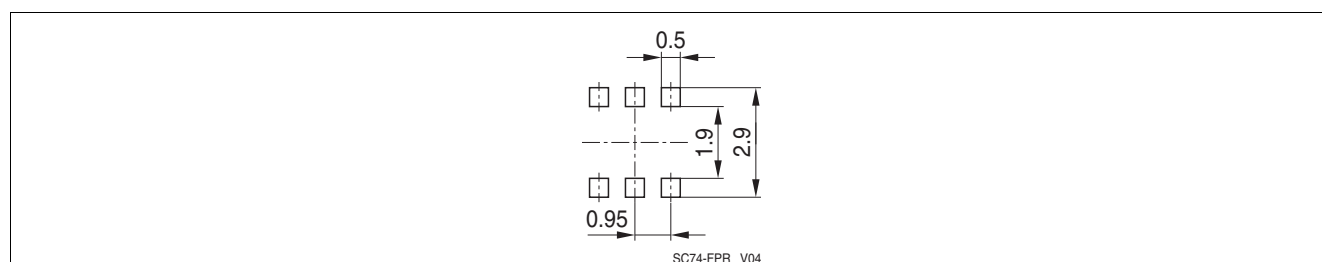
Figure 15 PG-SC74: Footprint
