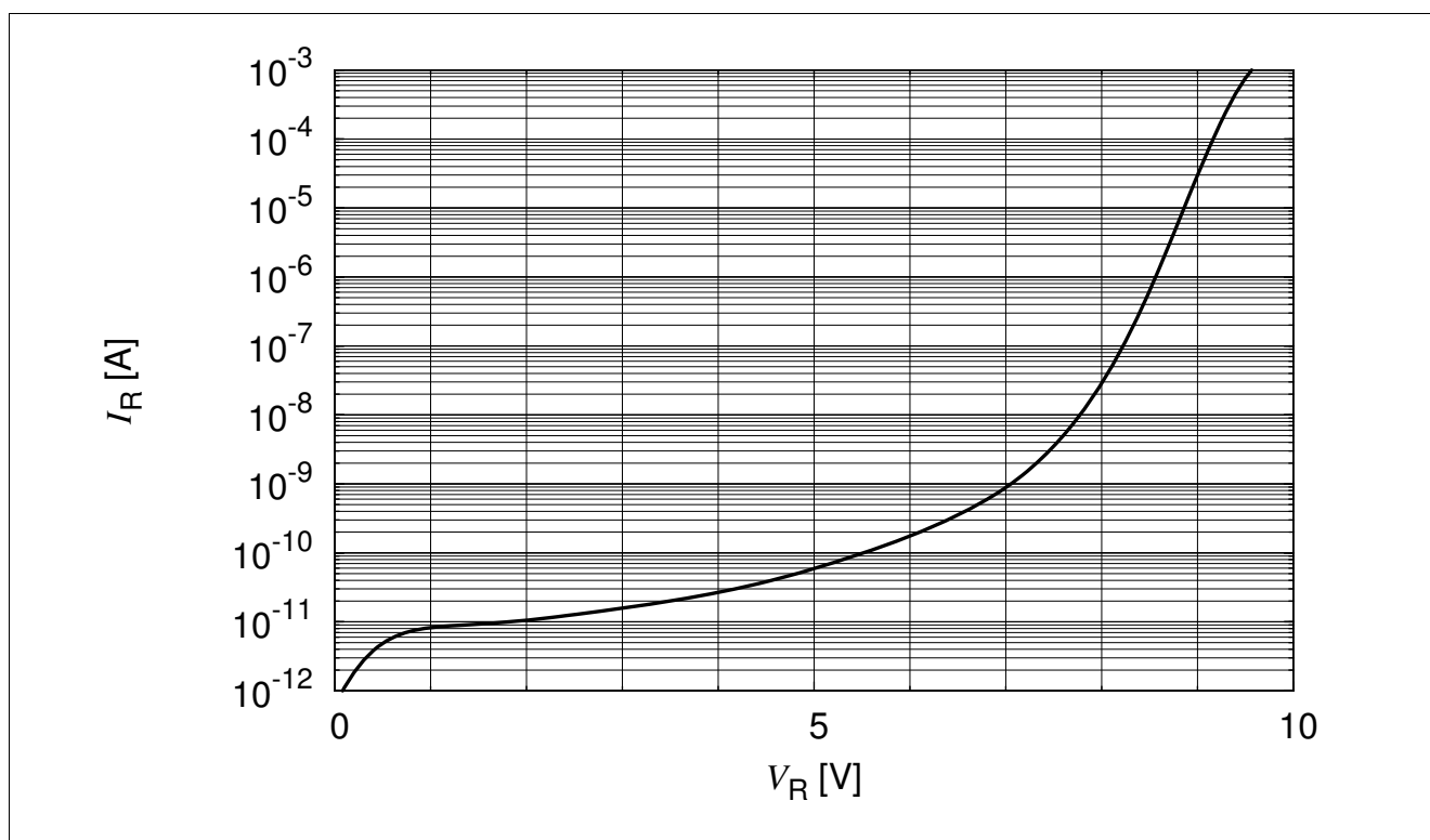
Figure 8 Reverse characteristic, I_R = f(V_R) , voltage forced
