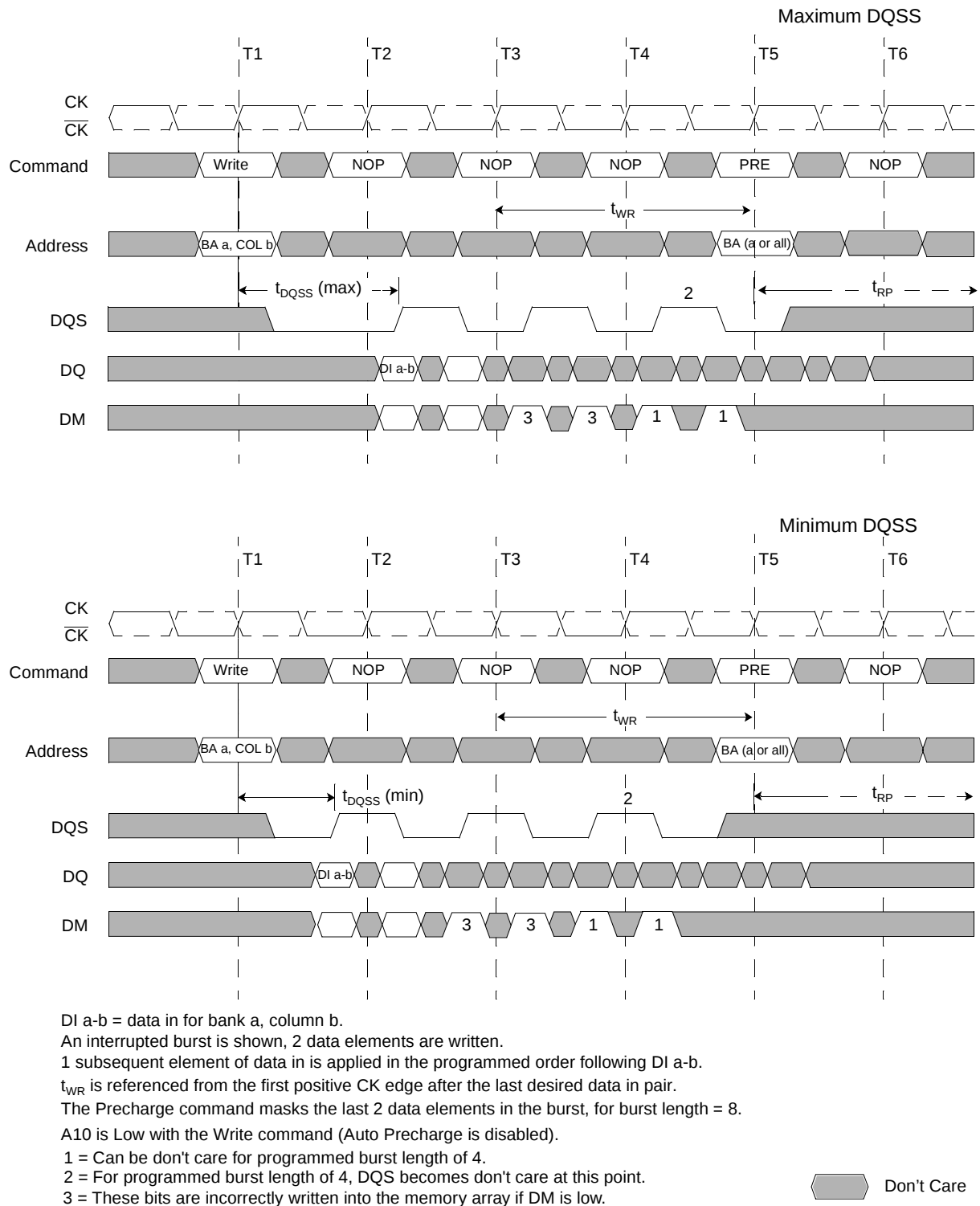
Figure 22 Write to Precharge: Interrupting (Burst Length = 4 or 8)
