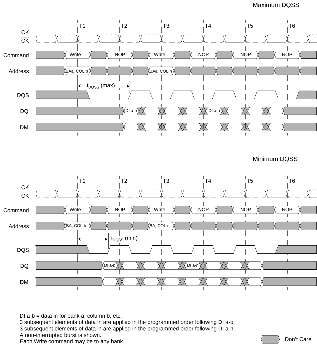
Figure 14 Write to Write (Burst Length = 4)
