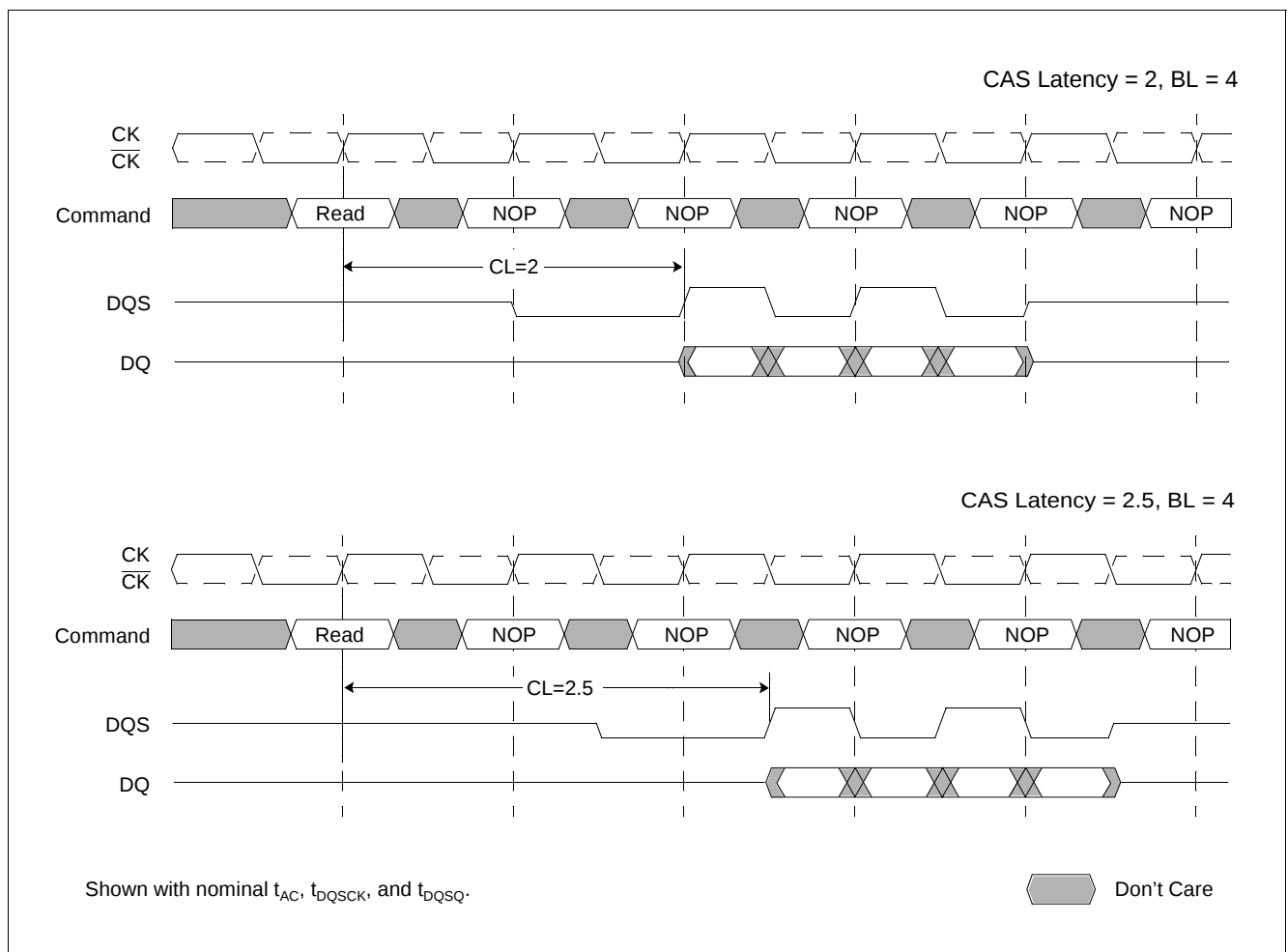
Figure 1 Required CAS Latencies
