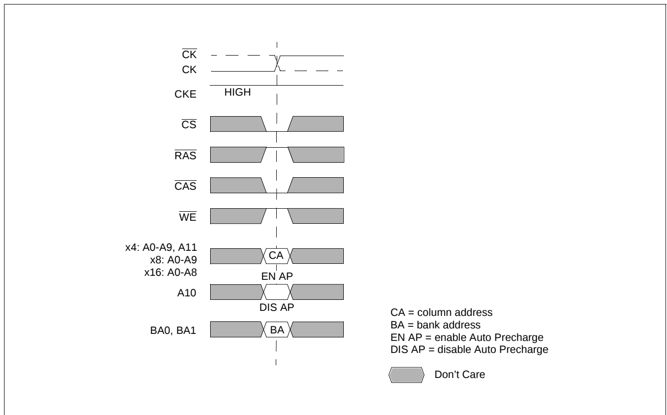
Figure 4 Read Command
