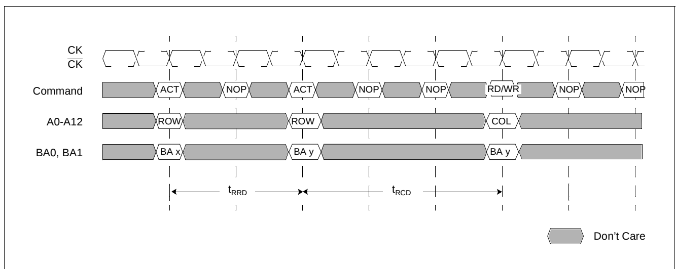
Figure 3 t_{\text{RCD}} and t_{\text{RRD}} Definition
