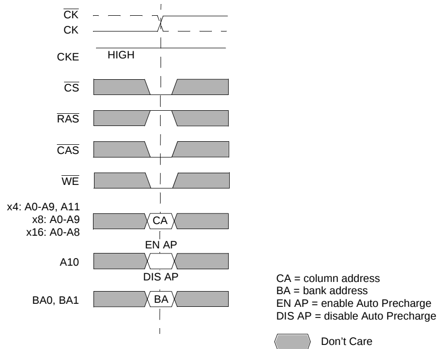
Figure 12 Write Command
