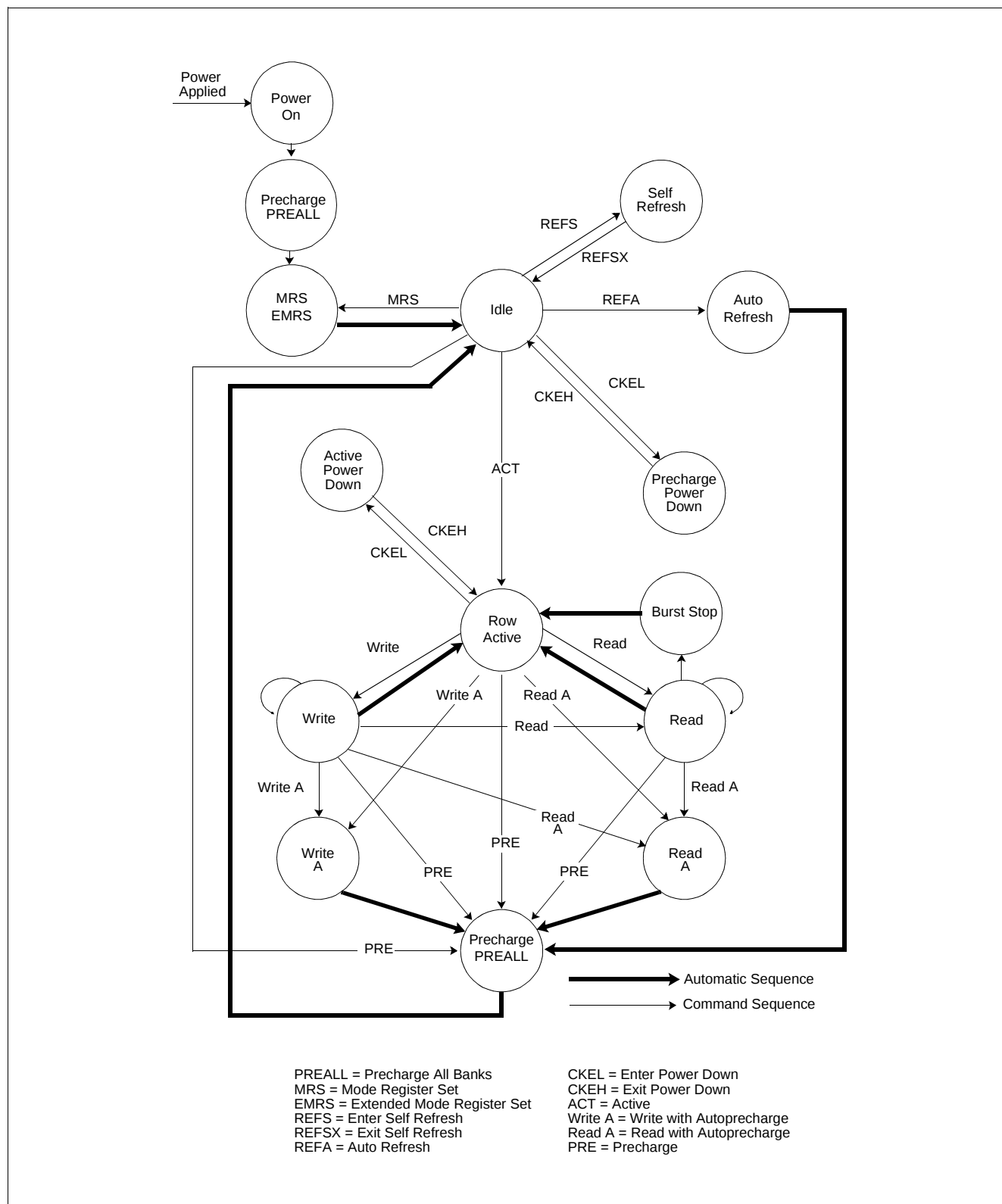
Figure 27 Simplified State Diagram
