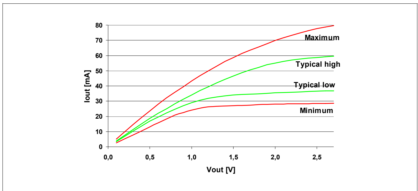
Figure 30 Weak Strength Pull-down Characteristics
