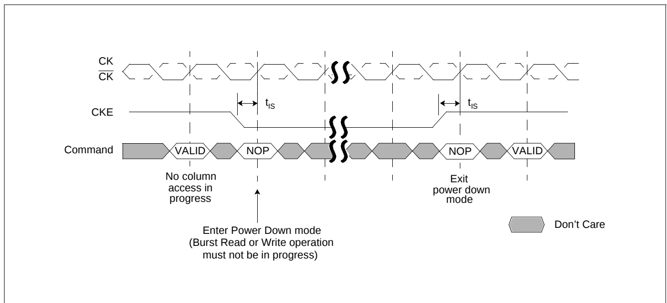
Figure 26 Power Down
