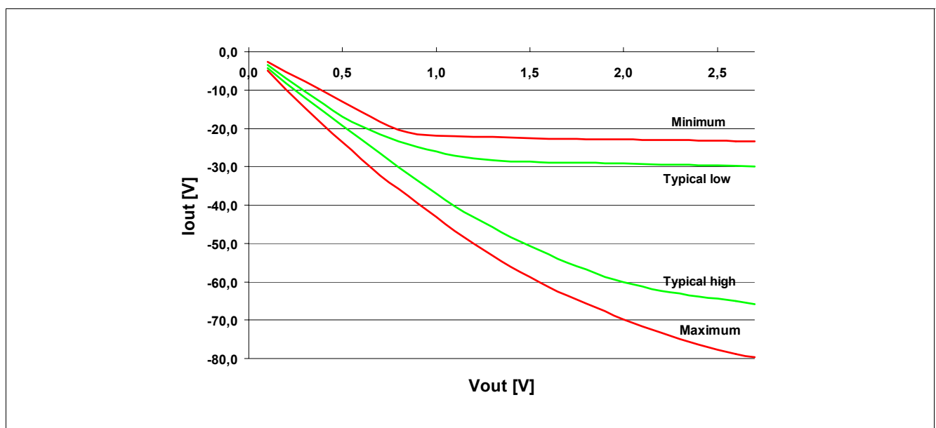
Figure 31 Weak Strength Pull-up Characteristics
