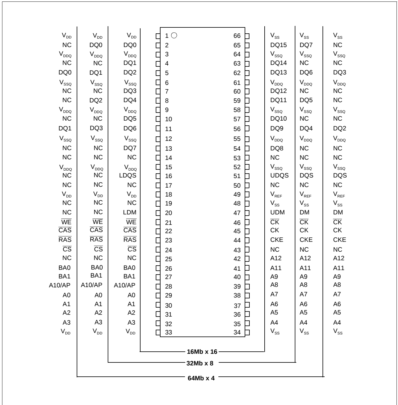
Figure 2 Pin Configuration P-TSOPII-66
