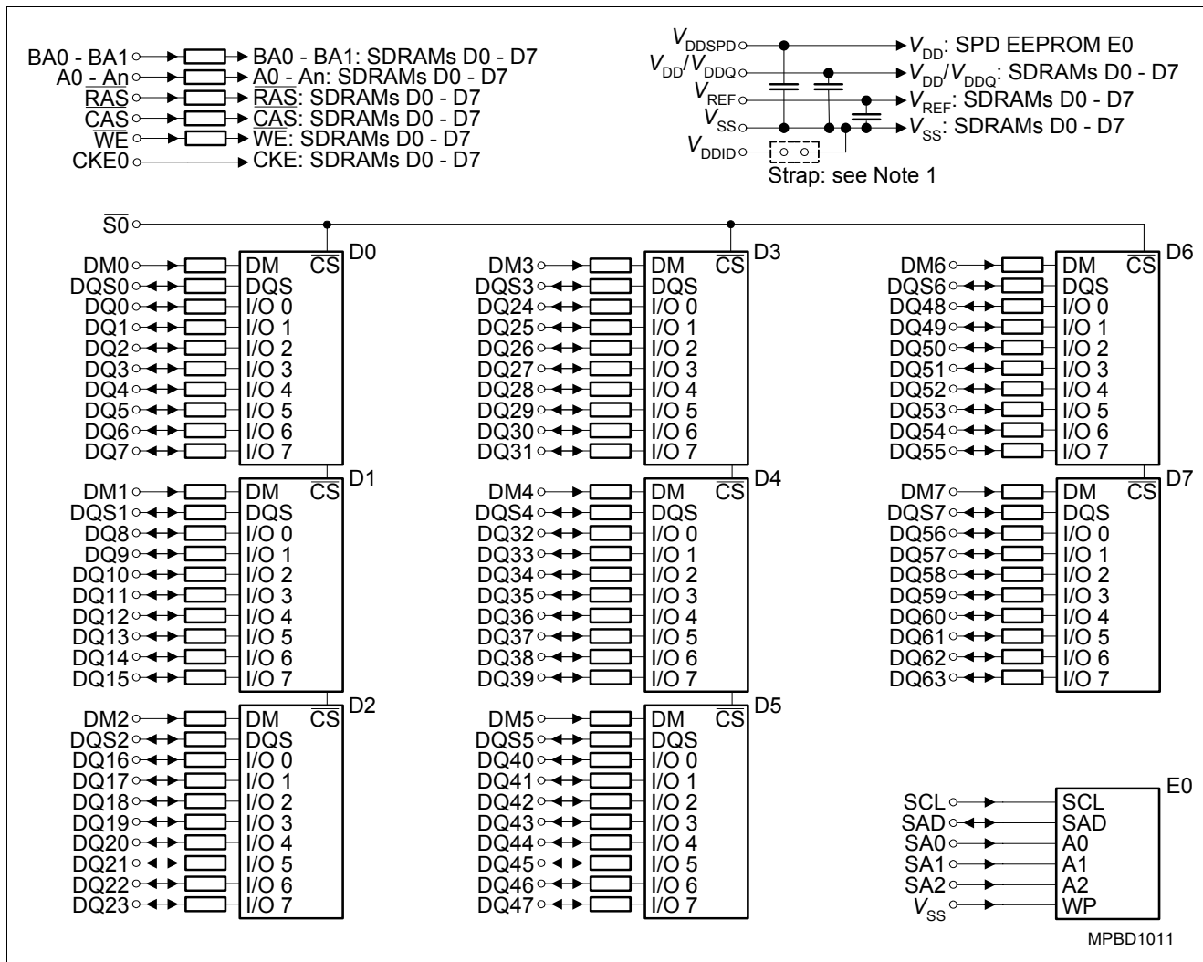
Figure 3 Block Diagram UDIMM Raw Card A (x64, 1 Rank, x8)
