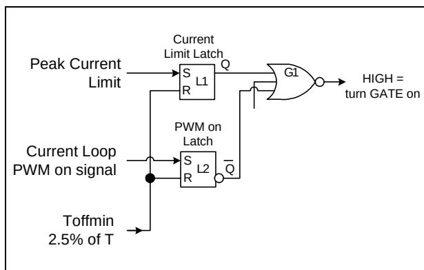
Figure 14 PWM Logic
