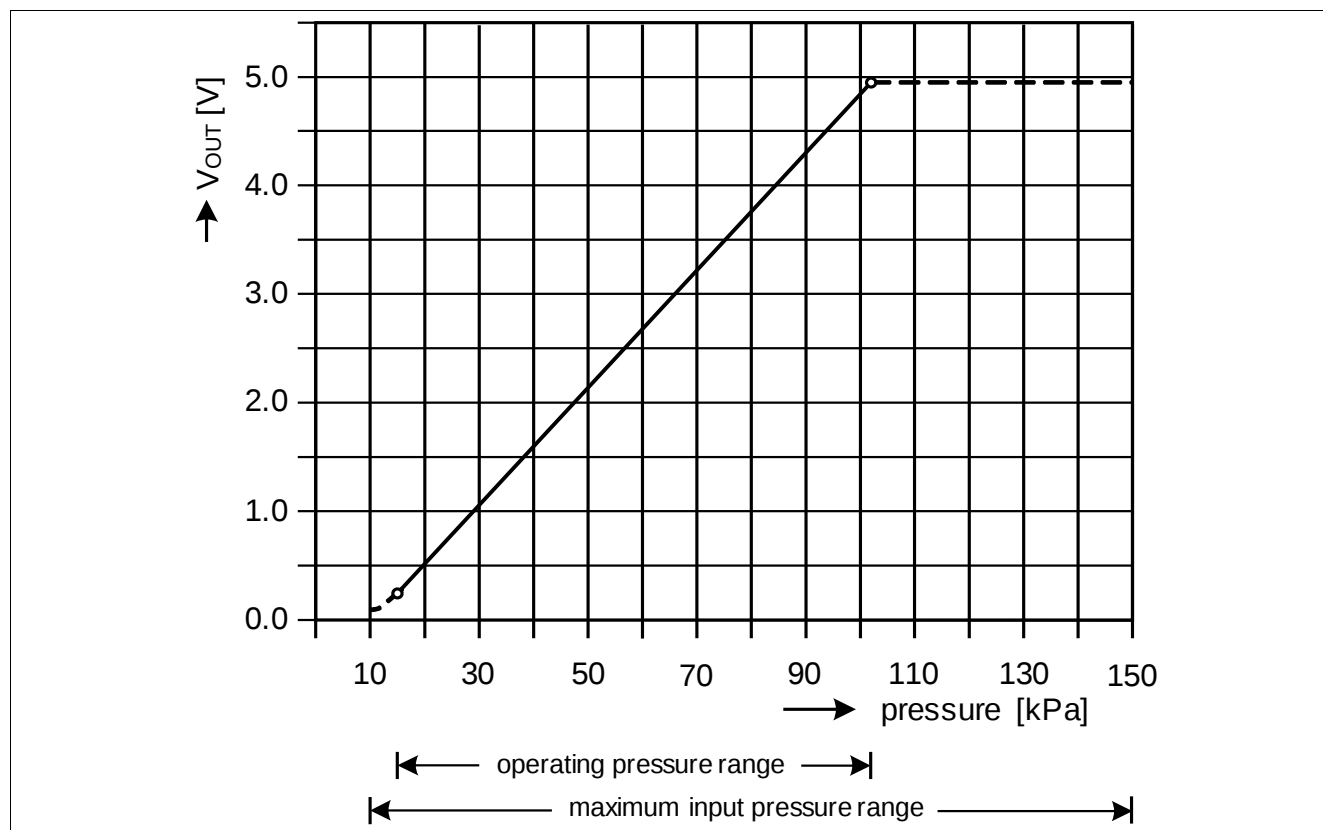
Figure 3 Transfer function
