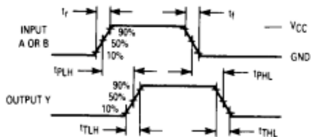
Figure 1 Switching Waveforms.
