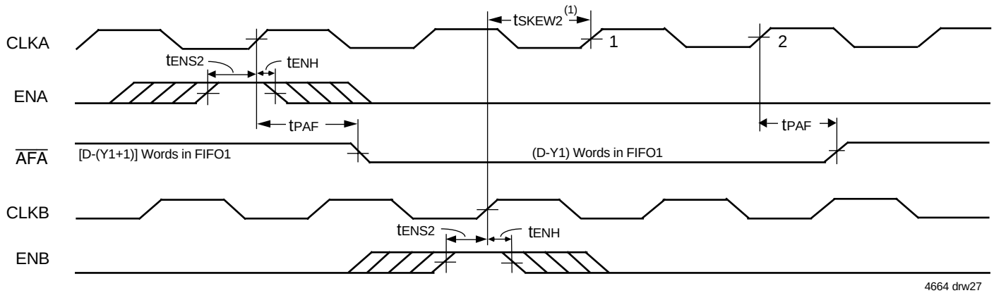
Figure 24. Timing for AEA when FIFO2 is Almost-Empty (IDT Standard and FWFT Modes)
