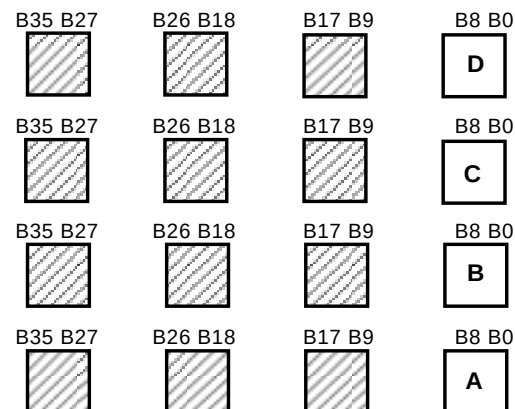
Figure 2. Bus Sizing
