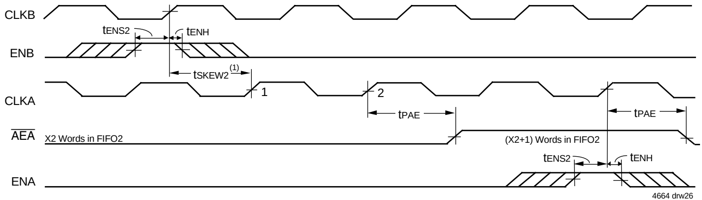
Figure 23. Timing for AEB when FIFO1 is Almost-Empty (IDT Standard and FWFT Modes)
