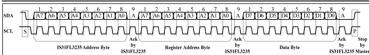
Figure 4 Writing to IS31FL3235(Typical)
