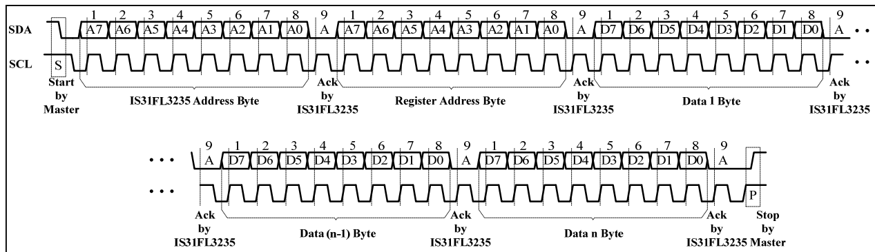
Figure 5 Writing to IS31FL3235(Automatic address increment)
