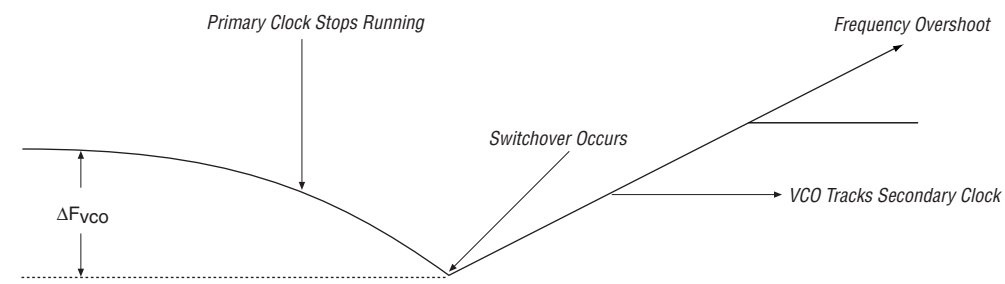
Figure 5-17. VCO Switchover Operating Frequency
