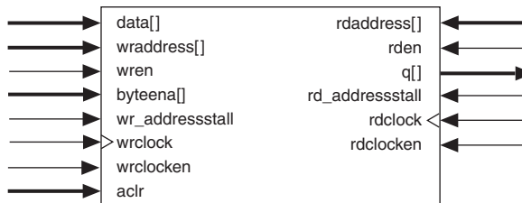
Figure 3-9. Cyclone III Device Family Simple Dual-Port Memory (1)
