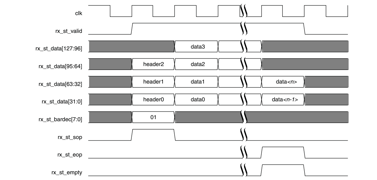
Figure 5–10. 128-Bit Avalon-ST rx\_st\_data<n> Cycle Definition for 3-DWord Header TLPs with QWord Aligned Addresses
