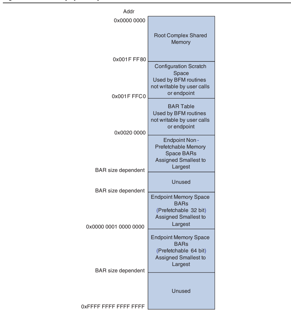
Figure 15-8. Memory Space Layout—No Limit
