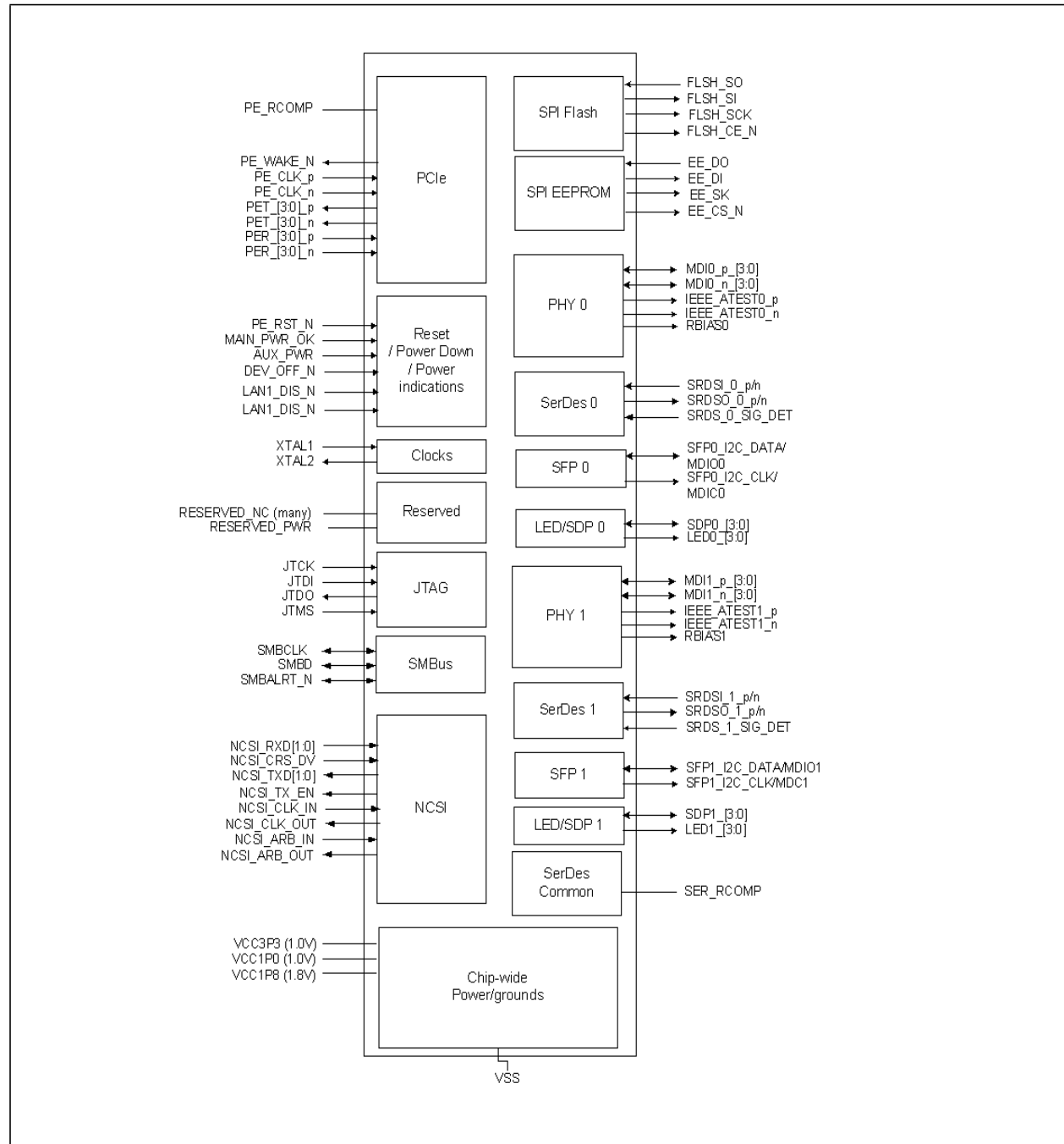
Figure 2-1. 82576 Interface Diagram
