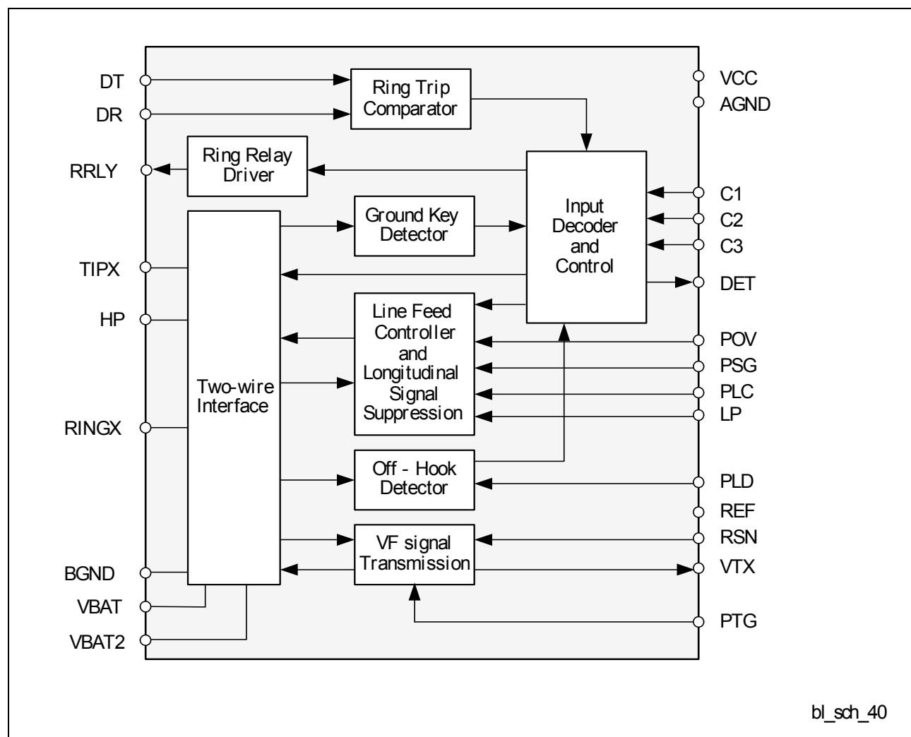
Figure 1 Block Diagram
