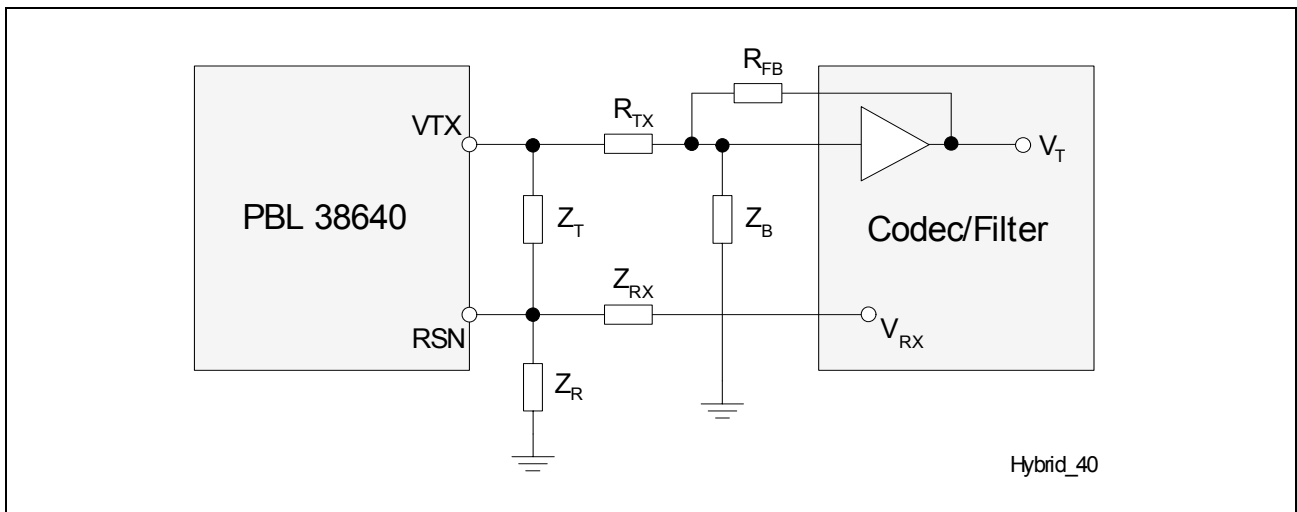
Figure 11 Hybrid Function
