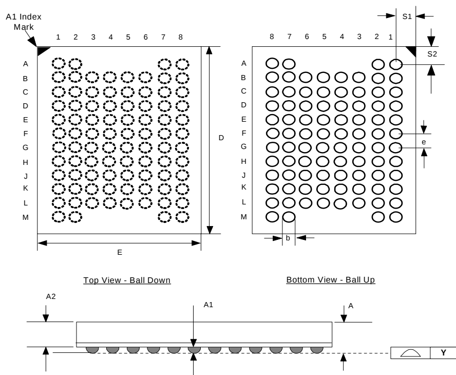
Figure 6. 1-Gbit, 88-ball (80 active) QUAD+ SCSP Specifications (11x11x1.4 mm)
