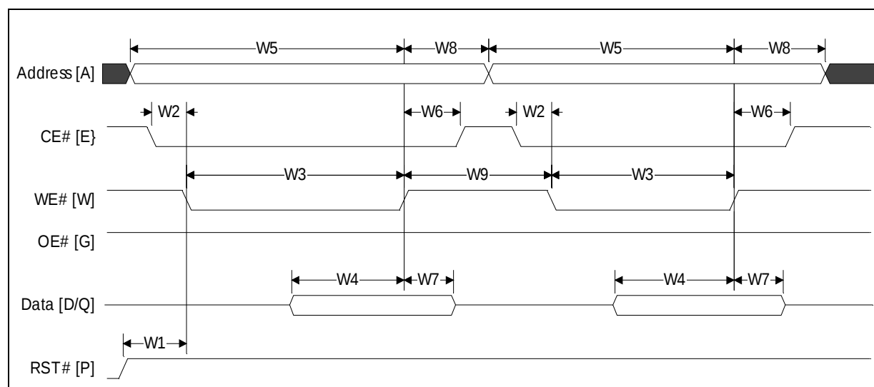
Figure 22. Write-to-Write Timing
