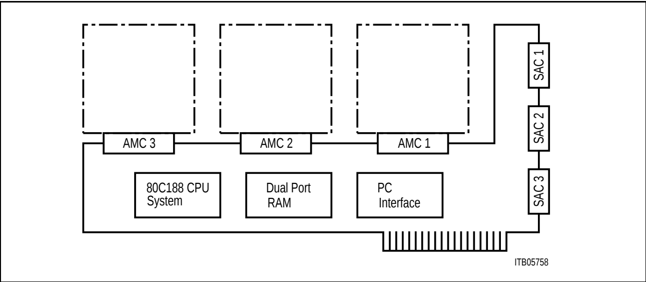
Figure 105 SIPB_5000 Mainboard
