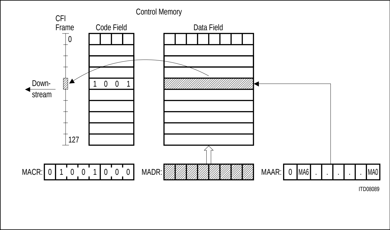
Figure 73 μP Access to the Downstream CFI Frame
