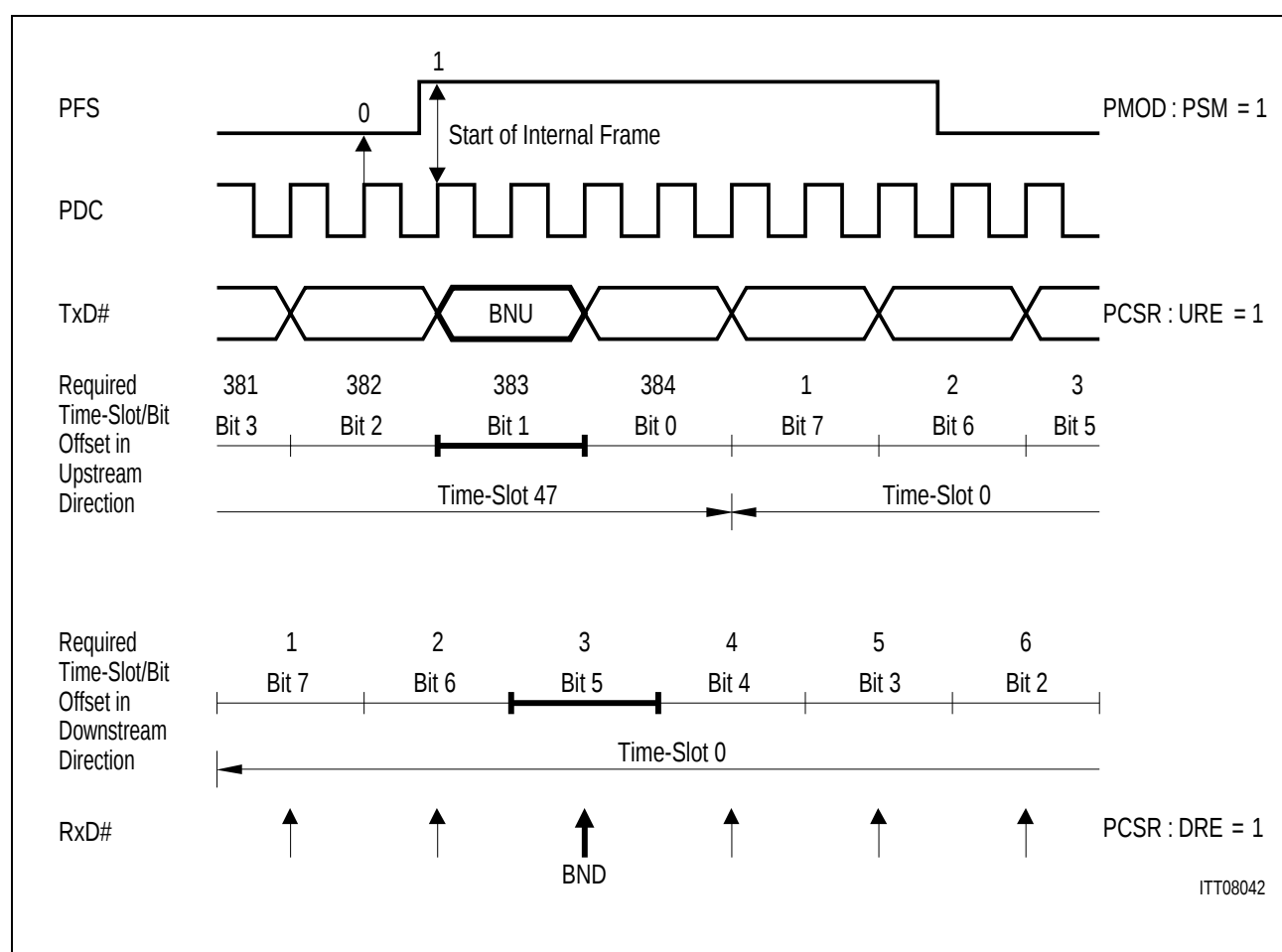
Figure 27 Timing for PCM Frame Offset of Example 2
