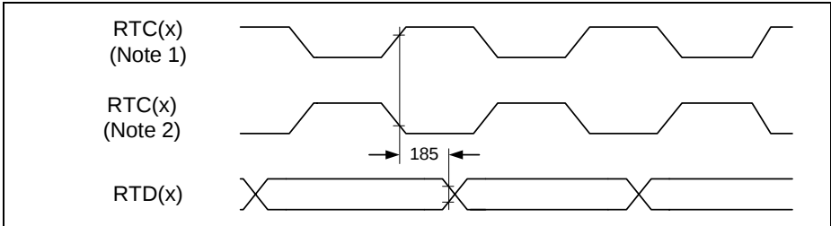
Figure 46 DS1/E1 Receive Data Timing
