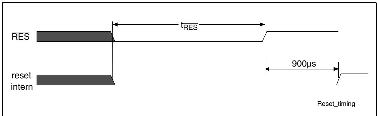
Figure 30 Reset Timing
