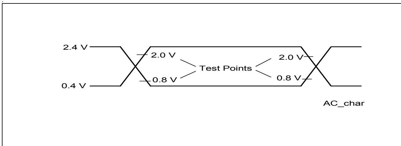
Figure 29 Input/Output Waveform for AC Tests
