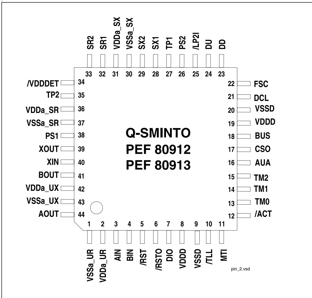
Figure 1 Pin Configuration
