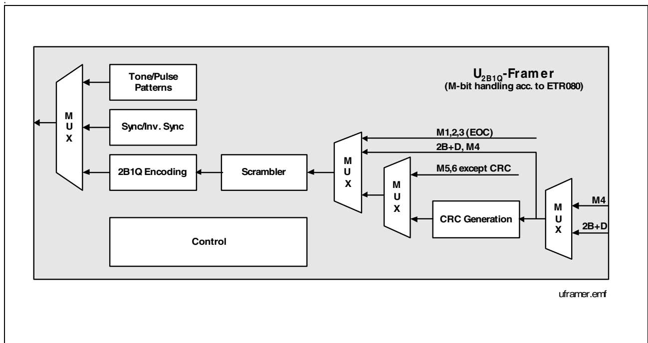
Figure 7 U 2B1Q Framing - Data Flow Scheme
