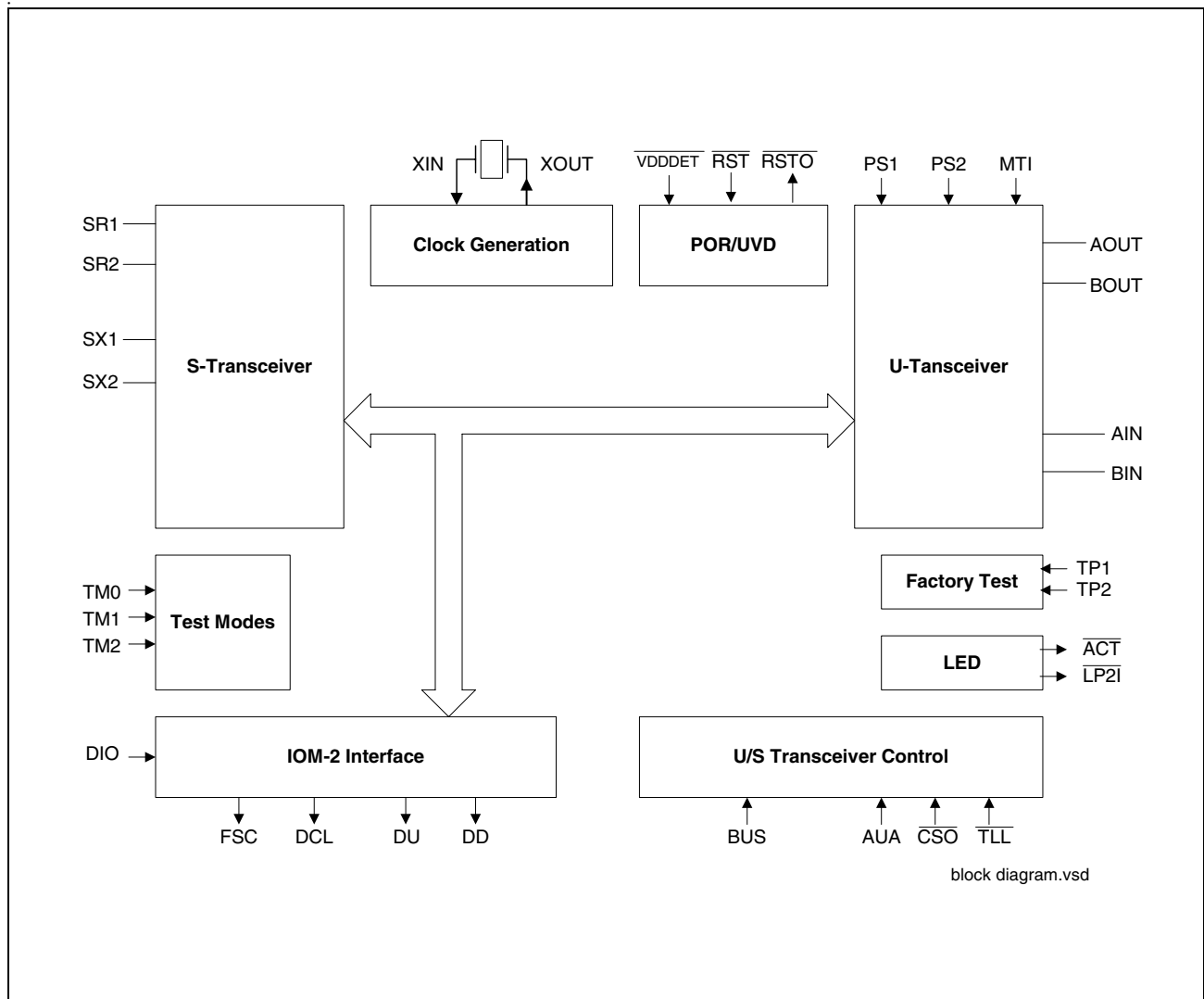
Figure 2 Block Diagram
