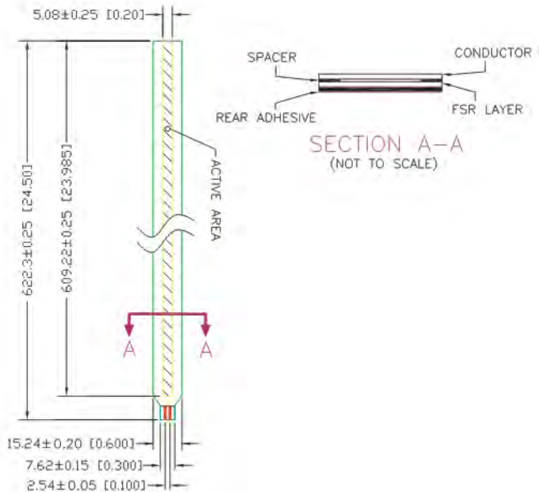
Figure 8: Model 408 Strip
