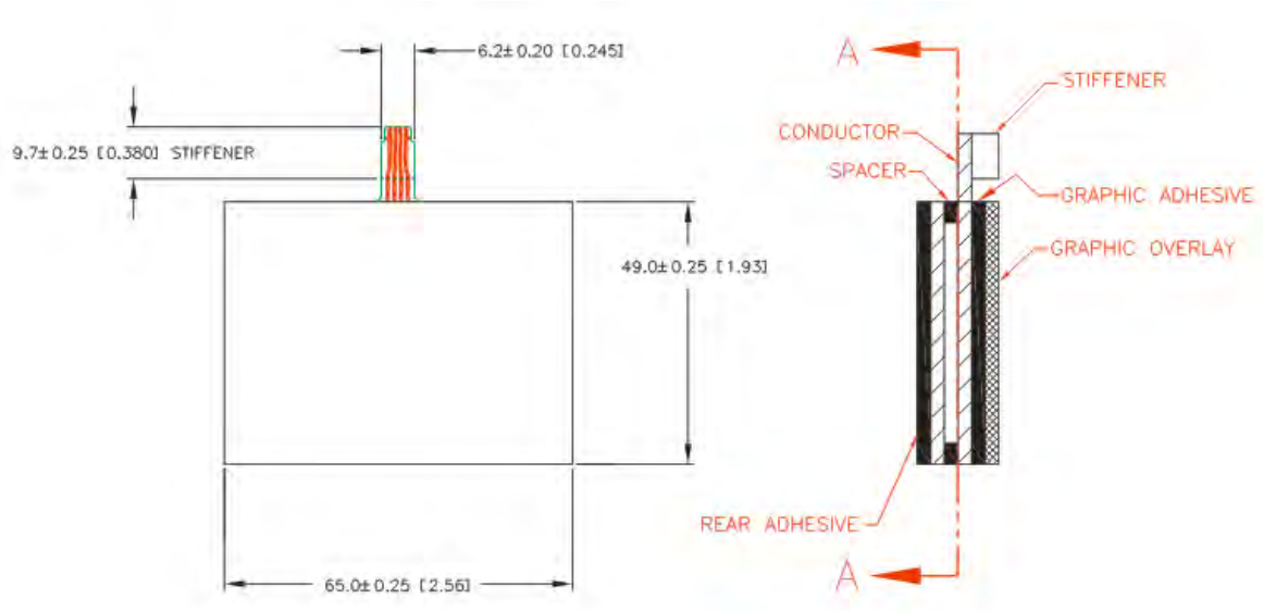
Figure 9: VersaPad Sensor
