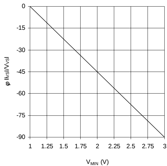
Graph 5. \phi I_{IVS}/V_{VS} vs V_{MIN} (IR21592/IR21593)
