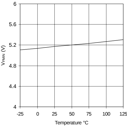
Graph 14. V FMIN vs Temperature (IR21592/IR21593)
