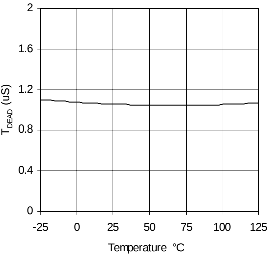
Graph 16. T DEAD vs Temperature (IR21593)
