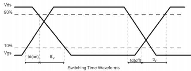
Figure 15. Switching waveform
