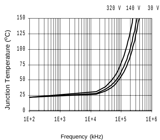
Figure 34. IR2111S T_J vs. Frequency (IRFPC50) R_{GATE} = 10 \Omega , V_{CC} = 15 V
