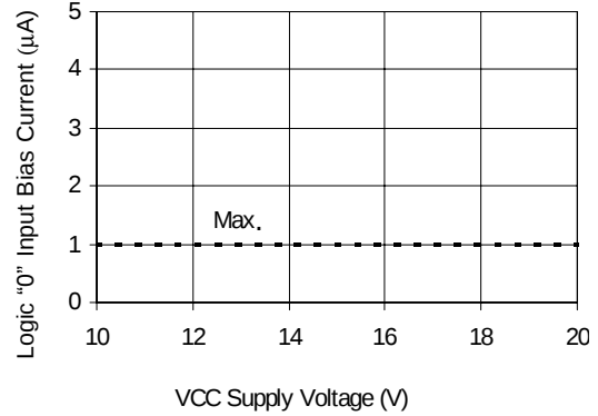
Figure 20B. Logic "0" Input Current vs. VCC Voltage
