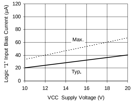
Figure 19B Logic "1" Input Current vs. VCC Voltage
