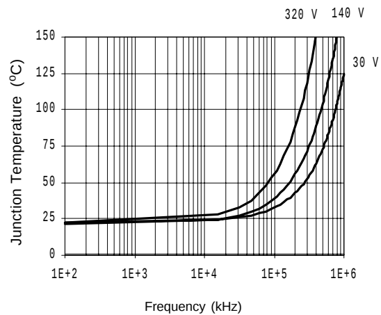
Figure 32. IR2111S T_J vs. Frequency (IRFBC30) R_{GATE} = 22 \Omega , V_{CC} = 15 V
