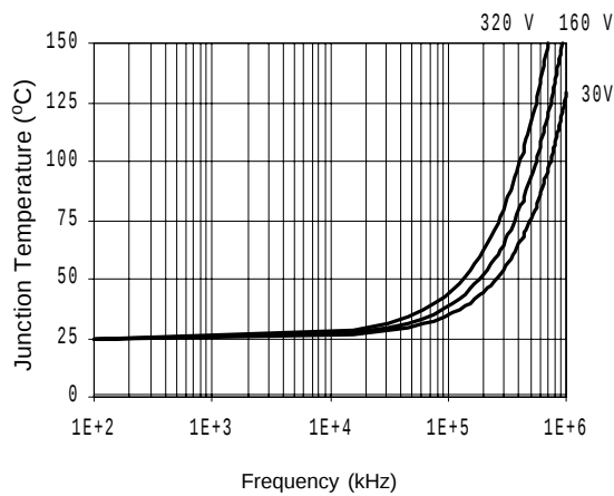
Figure 29. IR2111 T_J vs. Frequency (IRFBC40) R_{GATE} = 15 \Omega , V_{CC} = 15 V
