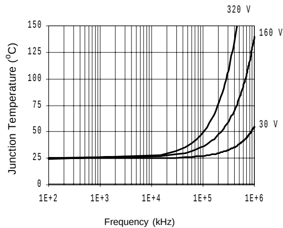
Figure 31. IR2111S T_J vs. Frequency (IRFBC20) R_{GATE} = 33 \Omega , V_{CC} = 15 V
