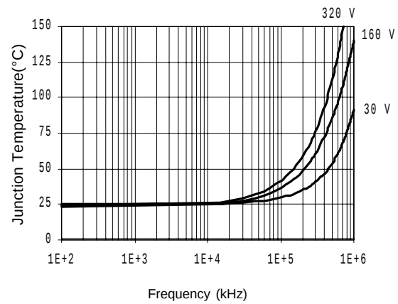
Figure 28. IR2111 T_J vs. Frequency (IRFBC30) R_{GATE} = 22 \Omega , V_{CC} = 15 V
