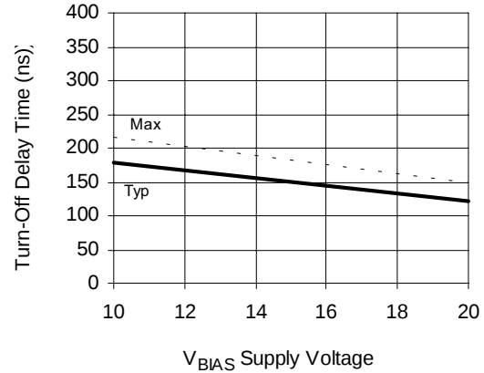
Figure 8B Turn-Off Time vs Voltage
