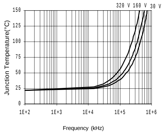
Figure 30. IR2111 T_J vs. Frequency (IRFPC50) R_{GATE} = 10 \Omega , V_{CC} = 15 V
