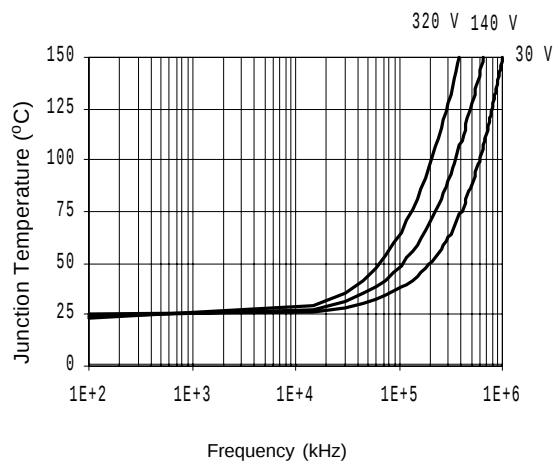
Figure 33. IR2111S T_J vs. Frequency (IRFBC40) R_{GATE} = 15 \Omega , V_{CC} = 15 V
