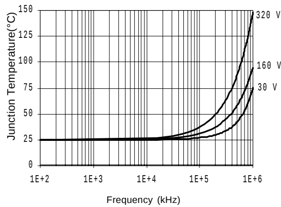
Figure 27. IR2111 T_J vs. Frequency (IRFBC20) R_{GATE} = 33 \Omega , V_{CC} = 15 V
