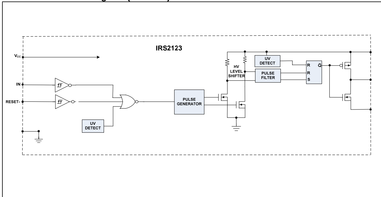
Functional Block Diagram (IRS2123)
