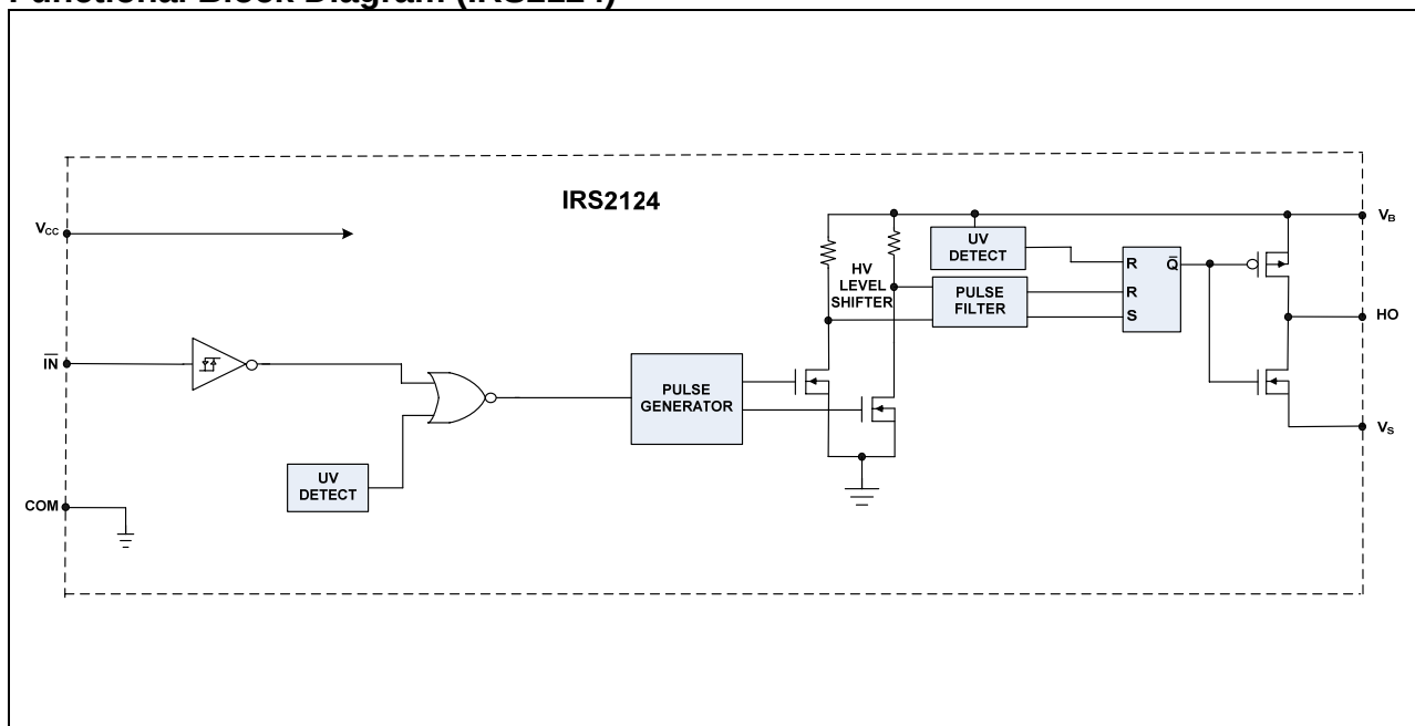
Functional Block Diagram (IRS2124)
