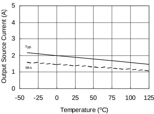
Figure 32A. Output Source Current vs. Temperature
