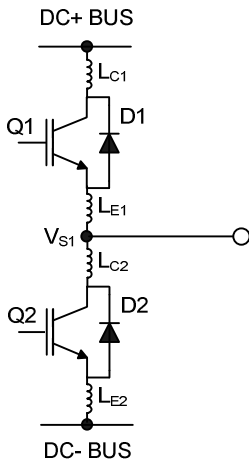
Figure 29: Parasitic Elements
