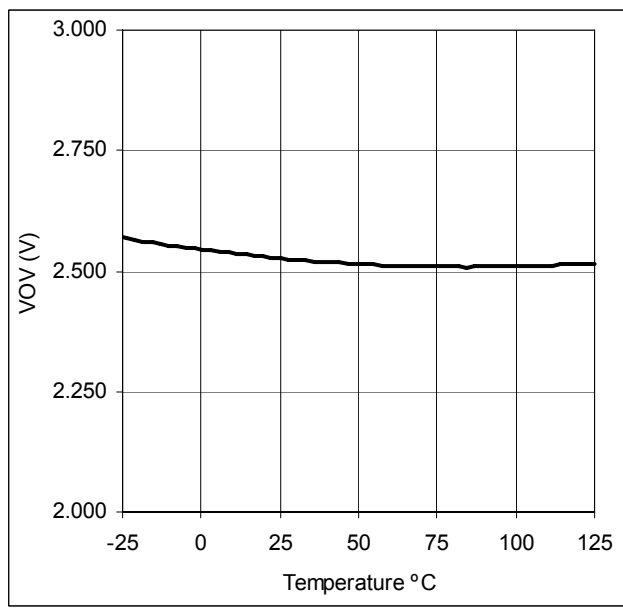
Fig. 14 VOV vs. Temperature
