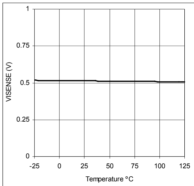
Fig. 12 VISENSE vs. Temperature
