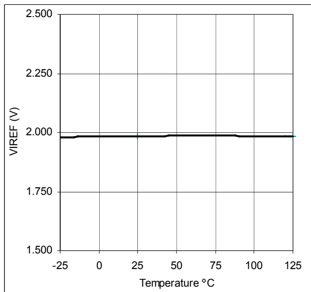
Fig. 11 VIREF vs. Temperature
