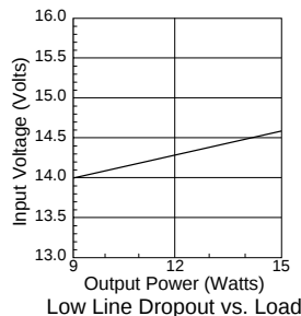
Low Line Dropout vs. Load
