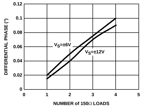
FIGURE 18. DIFFERENTIAL PHASE
