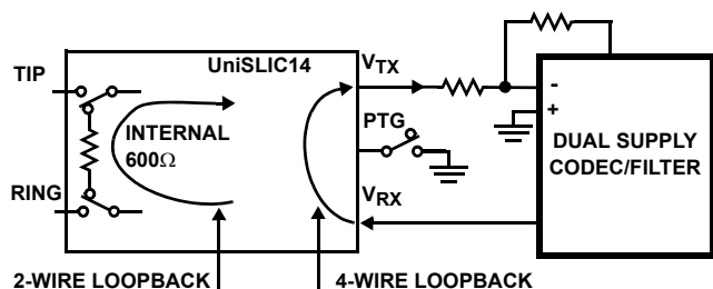
FIGURE 22. 4-WIRE AND 2-WIRE LOOPBACK TESTS
