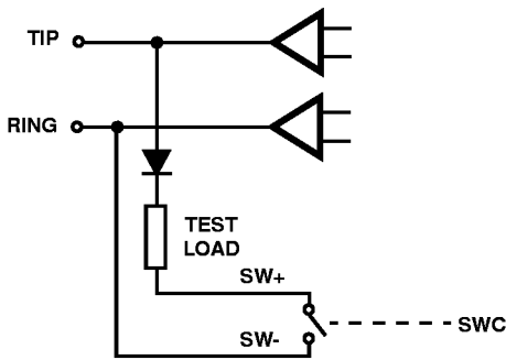
FIGURE 14. TEST LOAD SWITCHING
