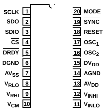
HI7190 20 LD SOIC, PDIP TOP VIEW
