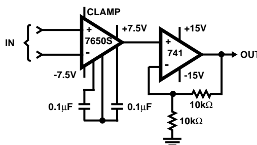
FIGURE 4. USING 741 TO BOOST OUTPUT DRIVE CAPACITY
