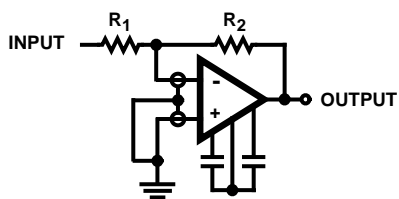
FIGURE 1A. INVERTING AMPLIFIER
