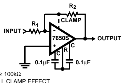
FIGURE 3. INVERTING AMPLIFIER WITH (OPTIONAL) CLAMP
