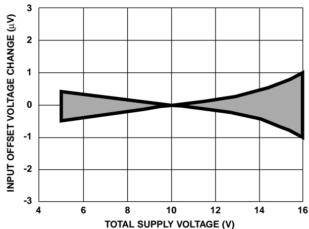
FIGURE 13. INPUT OFFSET VOLTAGE CHANGE vs SUPPLY VOLTAGE
