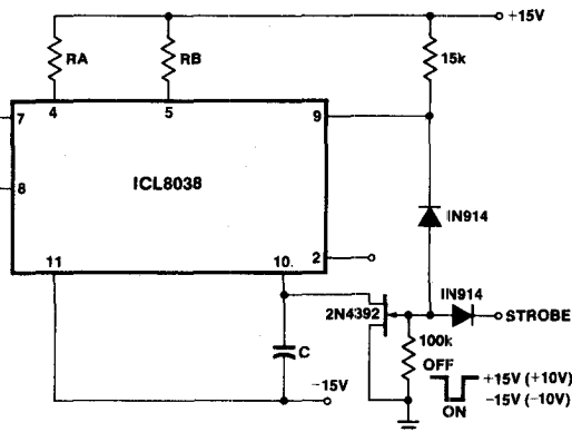
Figure 5: Strobe-Tone Burst Generator.
