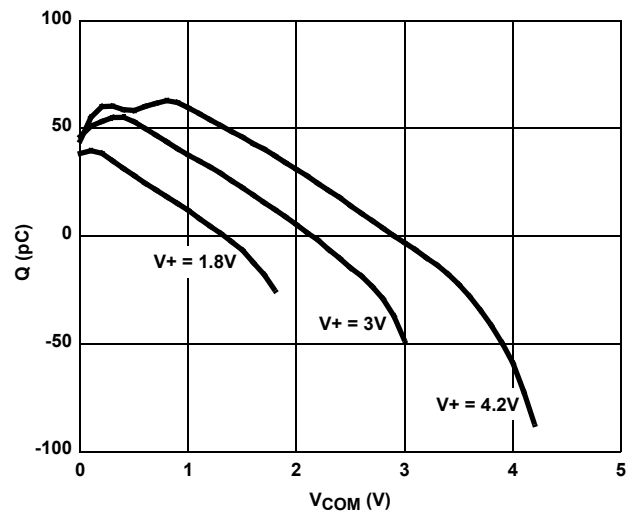
FIGURE 14. CHARGE INJECTION vs SWITCH VOLTAGE
