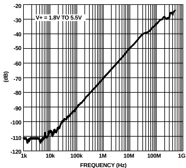
FIGURE 16. OFF ISOLATION
