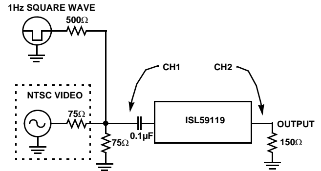
FIGURE 27. DC STEP RESPONSE CIRCUIT
