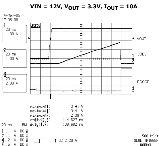
FIGURE 13. PG00D DELAY
