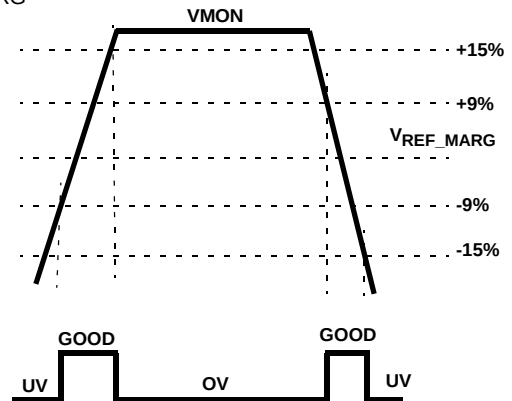
FIGURE 3. UNDERVOLTAGE-OVERVOLTAGE WINDOW
