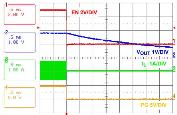
FIGURE 25. SOFT-DISCHARGE SHUTDOWN
