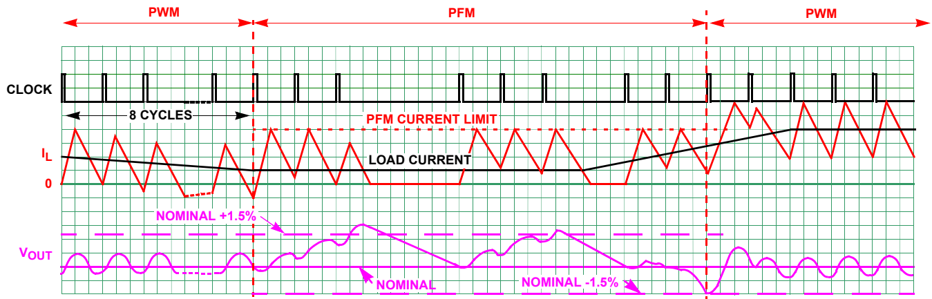
FIGURE 40. SKIP MODE OPERATION WAVEFORMS
