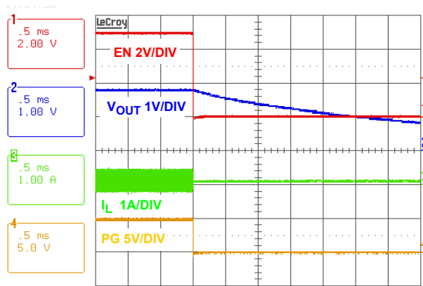
FIGURE 38. SOFT-DISCHARGE SHUTDOWN
