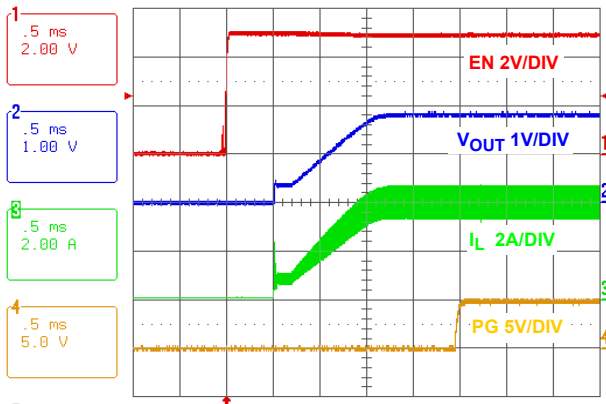
FIGURE 24. SOFT-START AT FULL LOAD
