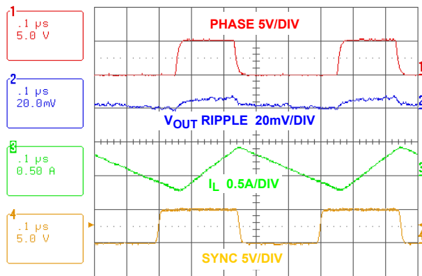
FIGURE 26. STEADY STATE OPERATION AT NO LOAD WITH FREQUENCY = 2MHz
